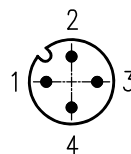
Contact arrangement
